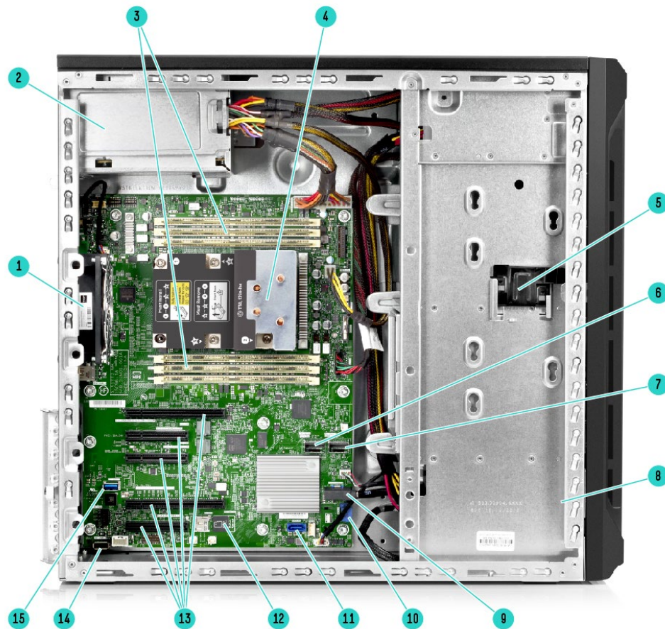
Internal View
